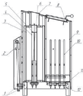
Fig. 4.1 Design of heater 10.0; 12.0; 16.0 kW
