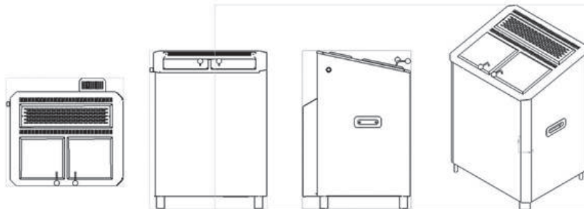
Fig. 2.1 Appearance of heater 10.0; 12.0; 16.0 kW
