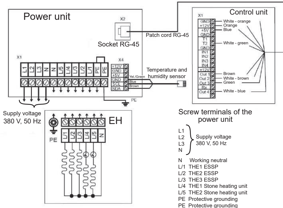
Fig. 6.2 Connection diagram for EH and CP 4.25 and 6.25 kW, 380 V
