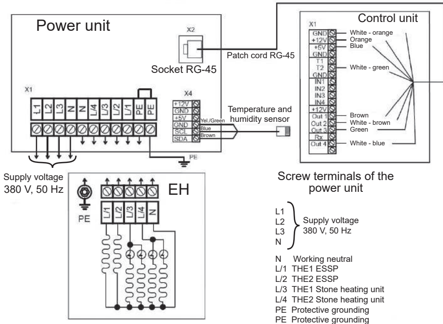
Fig. 6.3 Connection diagram for EH and CP 10.0; 12.0; 16.0 kW
