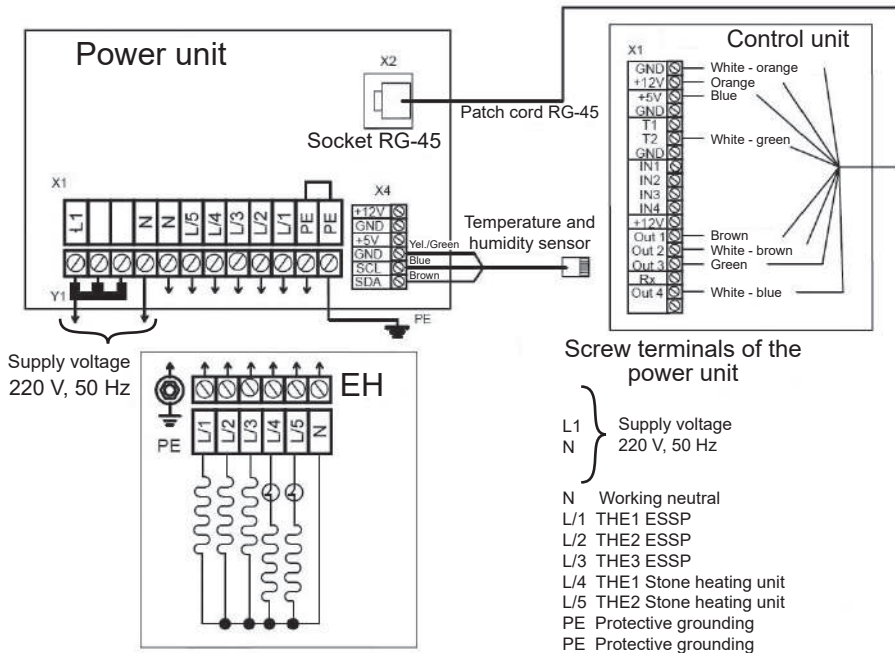
Fig. 6.1 Connection diagram for EH and CP 4.25 and 6.25 kW, 220 V
