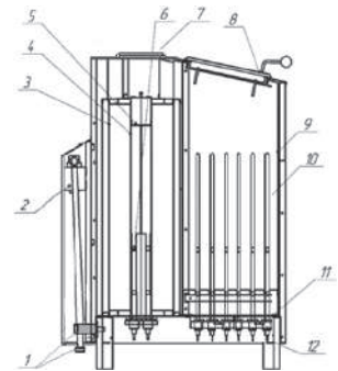
Fig. 4.2 Design of heater 18.0; 20.0; 22.0; 24.0 kW
