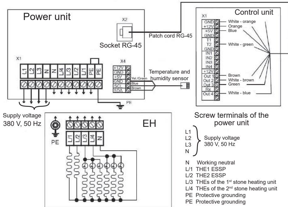
Fig. 6.4 Connection diagram for EH and CP 18.0; 20.0; 22.0; 24.0 kW
