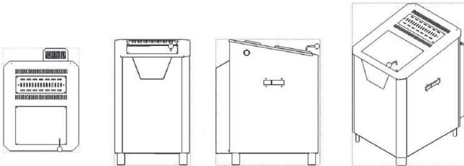
Fig. 1.1 Appearance of heater 4.25; 6.25 kW
